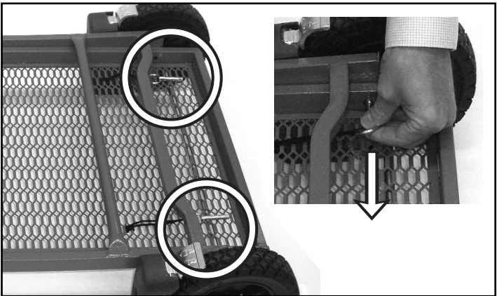
Step 2 Remove both locking pins.
