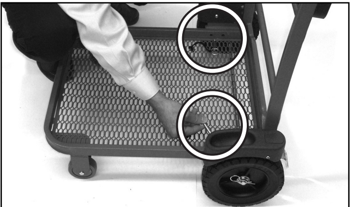
Step 4 Insert both locking pins to secure the frame to the base.
